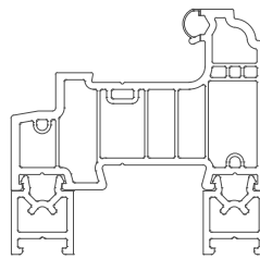
2153-001 LFS011 80MM FLUSH OUTER FRAME & 2156-001 20MM UNIVERSAL FRAME EXTENSION - LAN146
